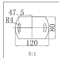
Footing dimensional drawing
